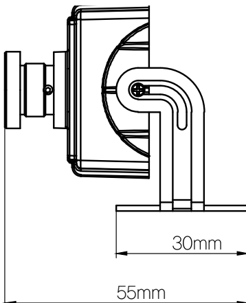
DC-V3213XJ-2.5mm - Side
